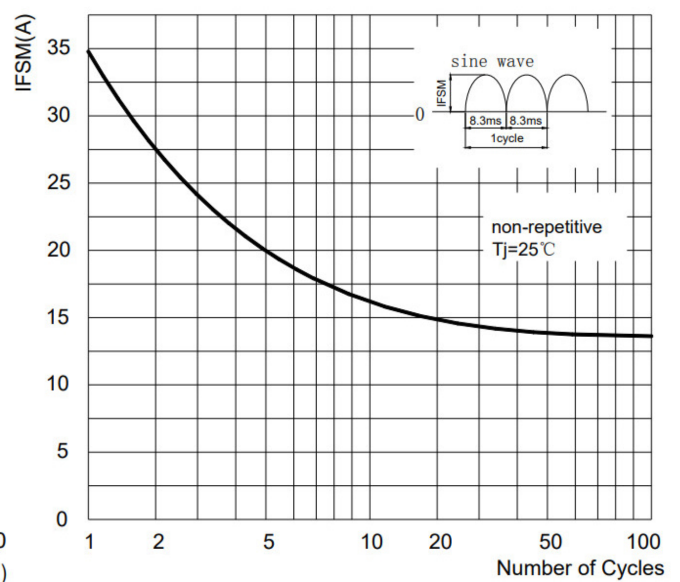
FIG.2: MAXIMUM NON-REPETITIVE FORWARD SURGE CURRENT
