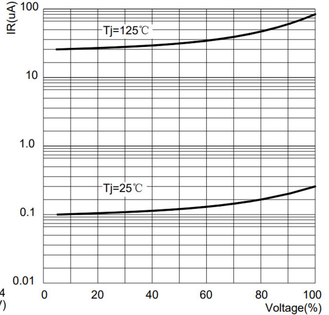
FIG.4: TYPICAL REVERSE CHARACTERISTICS
