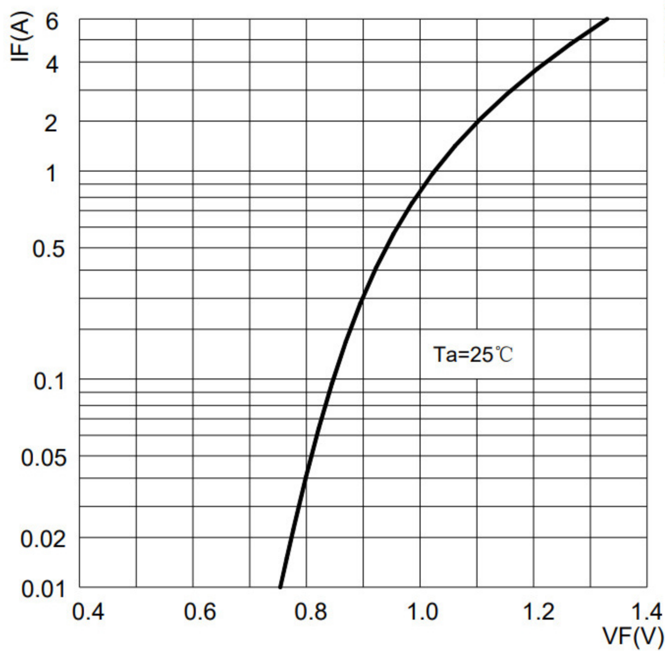
FIG.3: TYPICAL FORWARD CHARACTERISTICS
